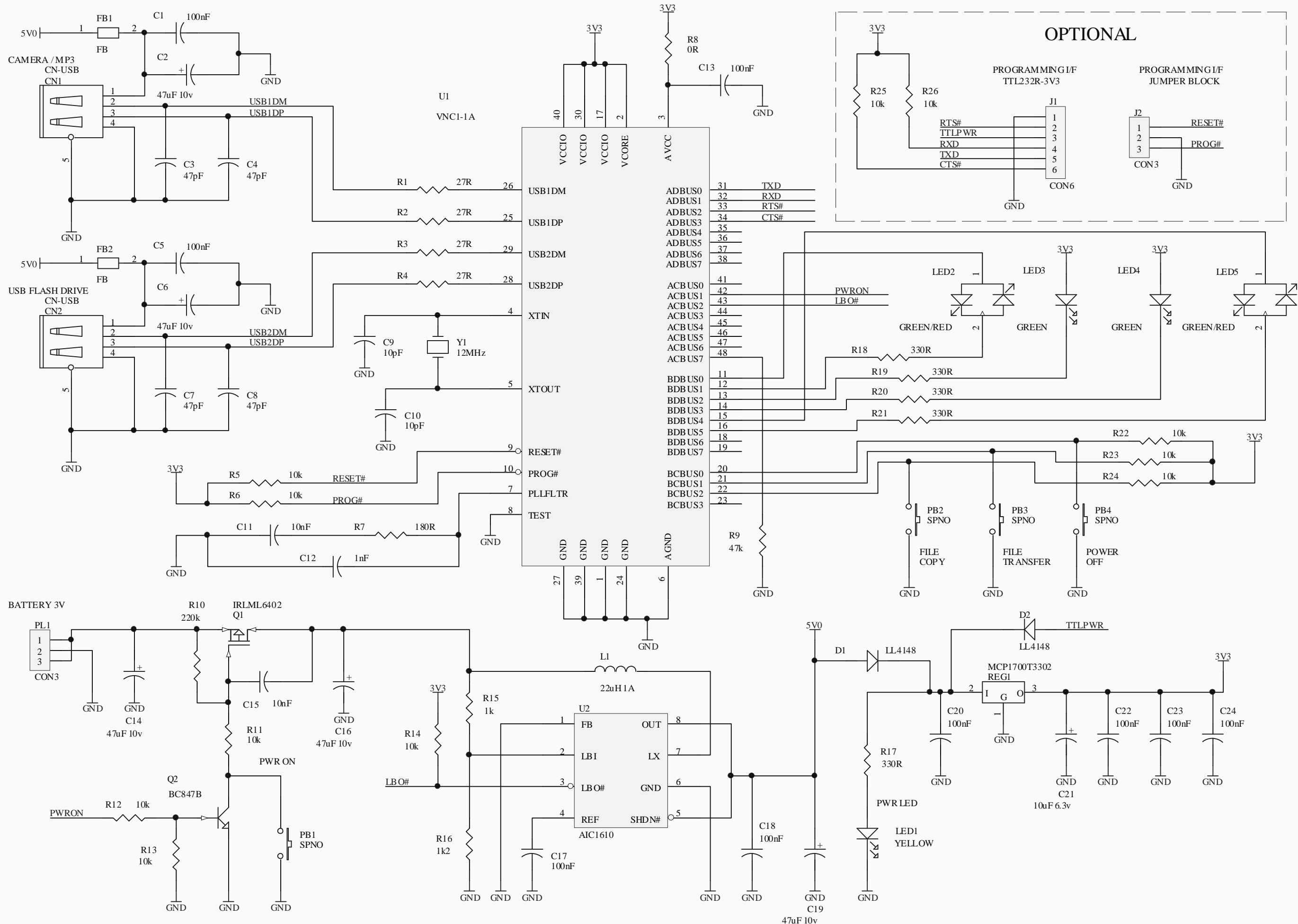
VINCULUM BACKUP FOR DIGITAL CAMERA / MP3 TO USB FLASH DRIVE SCHEMATIC
